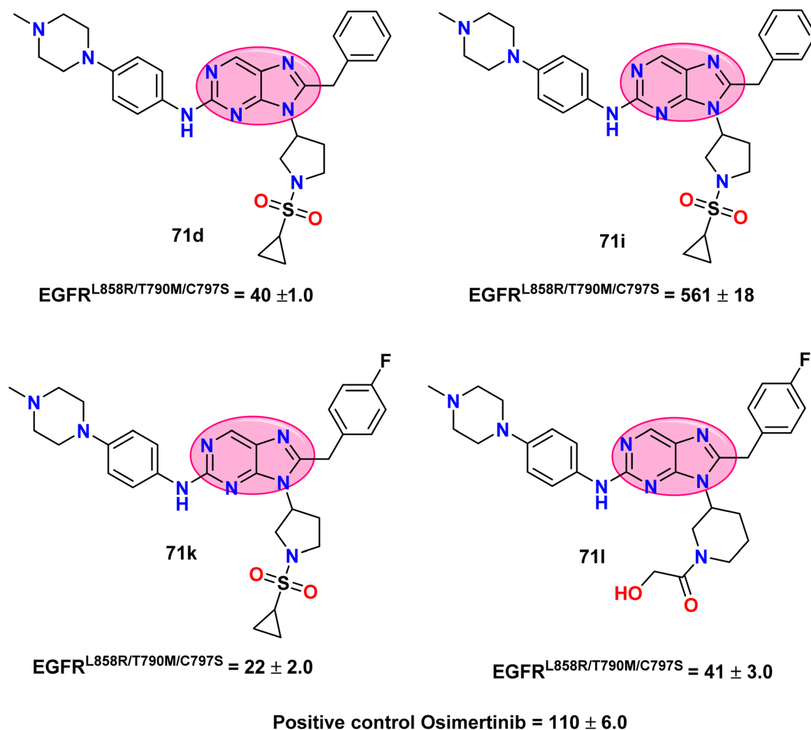
Fig. 3 Structures of the most active 9-heterocycl substituted 9H-purine derivatives and their values against the \text{EGFR}^{\text{L858R/T790M/C797S}} compared to osimertinib as a positive control.
