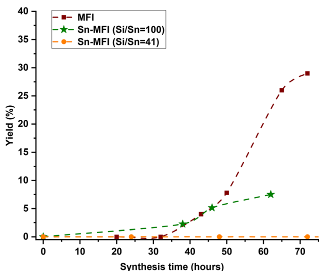
Fig. 3 Yield profiles of Si-MFI and Sn-MFI syntheses at 90 °C in FB. 1 \text{SiO}_2 \cdot X \text{ Sn}^{-1} : 0.5 \text{ TPAOH} : 20 \text{ H}_2\text{O} , where X = 100 or 41, from Sn and Si sources, tin chloride pentahydrate and TEOS, respectively. Samples were extracted along the synthesis and yield values were calculated through the extrapolation. The dashed line only serves as a guide to the eye.
