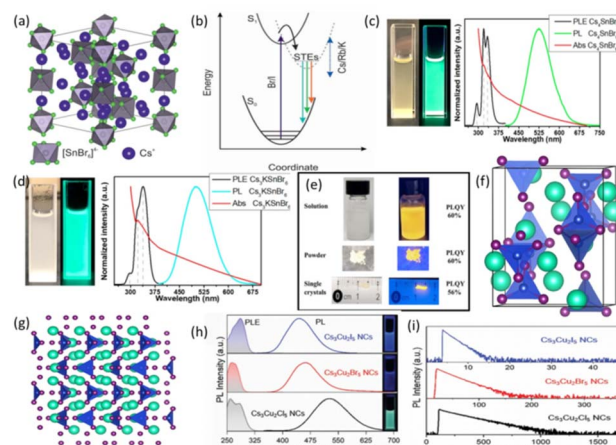
Fig. 5 (a) The crystal structure of \text{Cs}_4\text{SnBr}_6 viewed along the (111) axis with [\text{SnBr}_6]^{4-} octahedra (gray with green bromine atoms) separated by \text{Cs}^+ cations (blue). 4 Copyright 2018 Wiley-VCH. (b) Configurational coordinate diagram illustrating the origin of STE PL in \text{Cs}_{4-x}\text{A}_x\text{Sn}(\text{Br}_{1-y}\text{I}_y)_6 . 4 Copyright 2018 Wiley-VCH. PL, PLE, and Abs of (c) \text{Cs}_4\text{SnBr}_6 and (d) \text{Cs}_3\text{KSnBr}_6 perovskites. Photographs of colloidal NCs captured under daylight and 302 nm UV light, respectively. 30 Copyright 2020 American Chemical Society. (e) Photographs of [\text{Na}(\text{DMSO})_2]_3\text{SbBr}_6 solution, powder, and single crystals with/without UV light. 71 Copyright 2022 Wiley-VCH. (f) and (g) Crystal structure of \text{Cs}_3\text{Cu}_2\text{I}_5 . 72 Copyright 2018 Wiley-VCH. (h) PLE and PL spectra of colloidal \text{Cs}_3\text{Cu}_2\text{X}_5 NC solutions in hexane. Right insets show photographs of \text{Cs}_3\text{Cu}_2\text{X}_5 NC solutions under UV lamp excitation with \lambda = 254 nm. 73 Copyright 2019 Wiley-VCH. (i) Time-resolved PL decay spectra of \text{Cs}_3\text{Cu}_2\text{X}_5 NC solutions. 73 Copyright 2019 Wiley-VCH.
