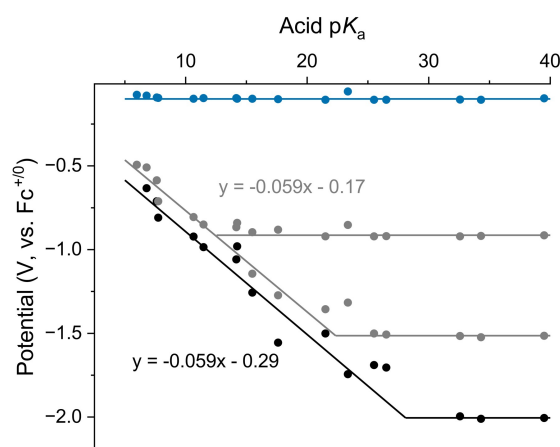
Figure 6. Potential- \text{pK}_a diagram of \text{V}_{\text{in}}\text{W}_{12} . Each data point represents an individual CV collected using 1 \text{ mM} \text{V}_{\text{in}}\text{W}_{12} and 4 \text{ mM} of the corresponding organic acid in MeCN. Reduction potentials are plotted against the \text{pK}_a of the organic acid used in each experiment. The horizontal lines represent the acid-independent redox events: the red, grey, and black traces denote the redox event at E_{1/2} = -0.30 \text{ V} , -1.80 \text{ V} and -2.31 \text{ V} respectively. The coloured diagonal lines represent the acid-dependent redox behaviour with the corresponding slopes; the blue line is for the vanadium-based reduction process, while grey and black lines correspond to the tungsten-based reduction events. The potentials were calibrated using \text{Fc}^{+/0} as the internal standard. All relevant CVs are compiled in Figure S29.
