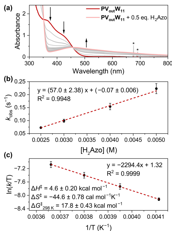
Figure 5. (a) Electronic absorption spectra of 0.5 mM \text{PV}_{\text{out}}\text{W}_{11} after addition of half an equivalent of \text{H}_2\text{Azo} over a 5-min period at room temperature. The sharp absorption, denoted with asterisks around 700 nm, indicates the injection of the \text{H}_2\text{Azo} stock solution. (b) Plot of k_{\text{obs}} as a function of [\text{H}_2\text{Azo}] with the concentration of \text{PV}_{\text{out}}\text{W}_{11} held constant at 0.25 mM at -30 \text{ }^{\circ}\text{C} . The concentration of \text{H}_2\text{Azo} is varied between 2.5 and 5 mM. (c) Eyring plot of the reaction of \text{PV}_{\text{out}}\text{W}_{11} (0.25 mM) and \text{H}_2\text{Azo} (2.5 mM) in MeCN between -30 and 0 \text{ }^{\circ}\text{C} . Y-axis adapts k_{\text{obs}} values.
