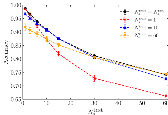
Fig. 5 Accuracy as a function of the number of active cells N_a = N_a^{\text{test}} , with \kappa_p = 0 and \kappa_a = 1500 . The black dots represent accuracy obtained from individual models, each trained using N_a^{\text{train}} = N_a^{\text{test}} . The red stars, blue triangles, and orange inverted triangles represent accuracy obtained from a single model trained with data for N_a = 1 , N_a = 15 or N_a = 60 , respectively. Each neural network is trained exclusively with local shape features.
