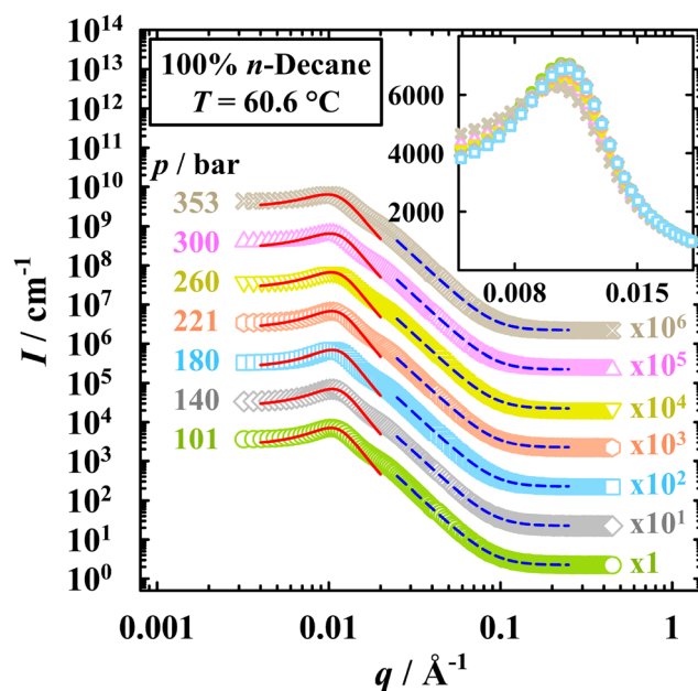
Fig. 4 Pressure-dependent bulk contrast SANS curves for the microemulsion system containing 100 wt% n -decane, recorded isothermally at T = 60.6\text{ °C} and \phi_c = 0.058 . Curves are displaced by a factor of 10 (101 bar unscaled). Peak region analyzed via the Teubner–Strey model 32 (red solid lines); high q analyzed with Porod's law, taking into account the diffuseness of the amphiphilic film 33,34 (blue dashed lines). Inset: Unscaled close-up of the peak region with linear I axis. Fits are omitted for better visibility.
