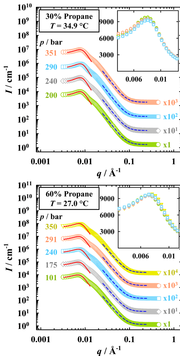
Fig. 6 Pressure-dependent bulk contrast SANS curves for the micro-emulsion system containing (top) 30 wt% propane, recorded isothermally at T = 34.9\text{ °C} and \phi_C = 0.042 , and (bottom) 60 wt% propane, recorded isothermally at T = 27.0\text{ °C} and \phi_C = 0.039 . Curves are displaced by a factor of 10 (lowest pressure unscaled). Peak region analyzed via the Teubner–Strey model 32 (red solid lines); high q analyzed with Porod's law, taking into account the diffuseness of the amphiphilic film 33,34 (blue dashed lines). Inset: Unscaled close-up of the peak region with linear I axis. Fits are omitted for better visibility.
