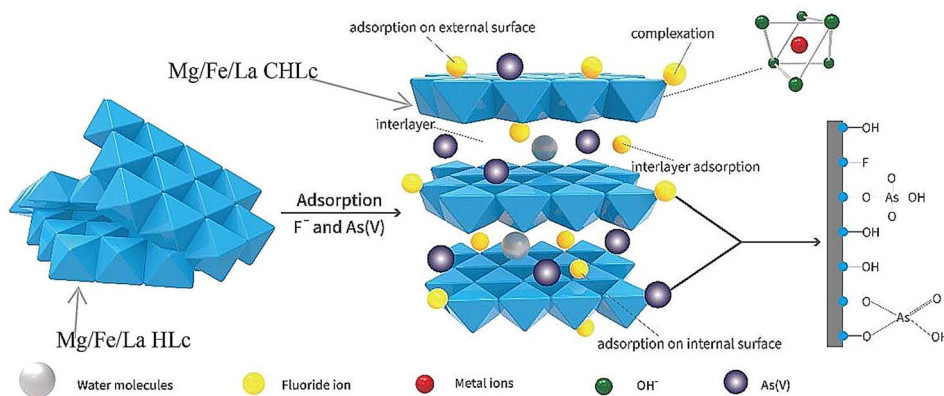
Fig. 18 MMO hydration mechanism for fluoride ion adsorption by MgFeLa- \text{MMO} . 28 Copyright 2018, American Chemical Society.
