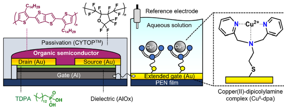
Fig. 40 Schematic of the extended-gate-type OFET for oxanion detection. The extended-gate electrode was functionalized with the \text{Cu}^{\text{II}} -dpa complex (reproduced with permission from ref. 156. Copyright 2022, ACS).
