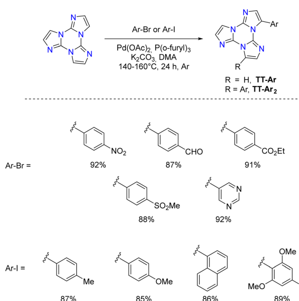
Scheme 9 Synthesis of TT derivatives by direct arylation.
