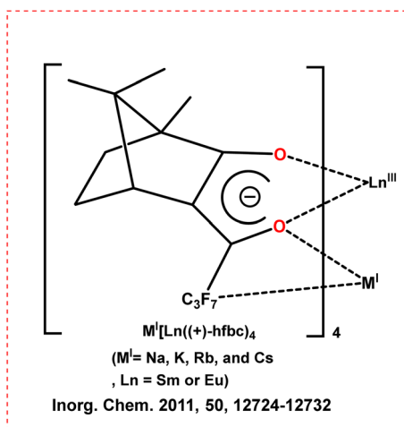
Scheme 5 Chemical structures of the ligands and Ln complexes ( \text{M}'[\text{Ln}((+)\text{-hfbcb})_4] ). 32
