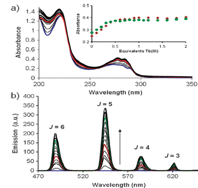
Scheme 20 (Above) Chemical structures of ligands 1 and 2. 75 (Below) (a) Changes in the UV-vis absorption spectrum of 1 (upon titration with Tb(CF 3 SO 3 ) 3 ) in CH 3 CN. Inset: The changes at 275 nm for 1 2 Tb and 2 2 Tb. (b) Corresponding changes in Tb(III) emission. Reproduced from ref. 75 with permission from the Royal Society of Chemistry, copyright [2011]. 75
