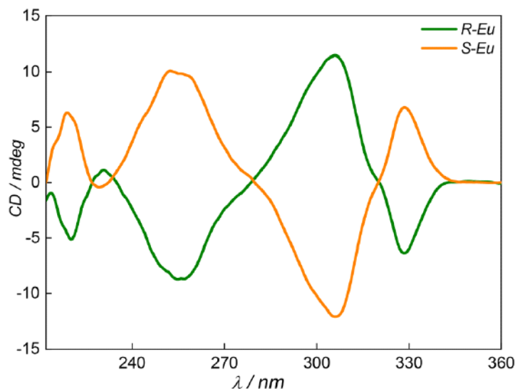
Scheme 46 (Above) Chemical structures of the ligands and Ln complexes ( R/S -Ln and R/S -Eu- \text{Ph}_3\text{PO} , \text{Ln} = \text{Eu, Gd} ), adapted from ref. 94. (Below) CD spectra of R/S -Eu in \text{CH}_3\text{OH} . Reproduced from ref. 94 with permission from the Royal Society of Chemistry, copyright [2024]. 94
