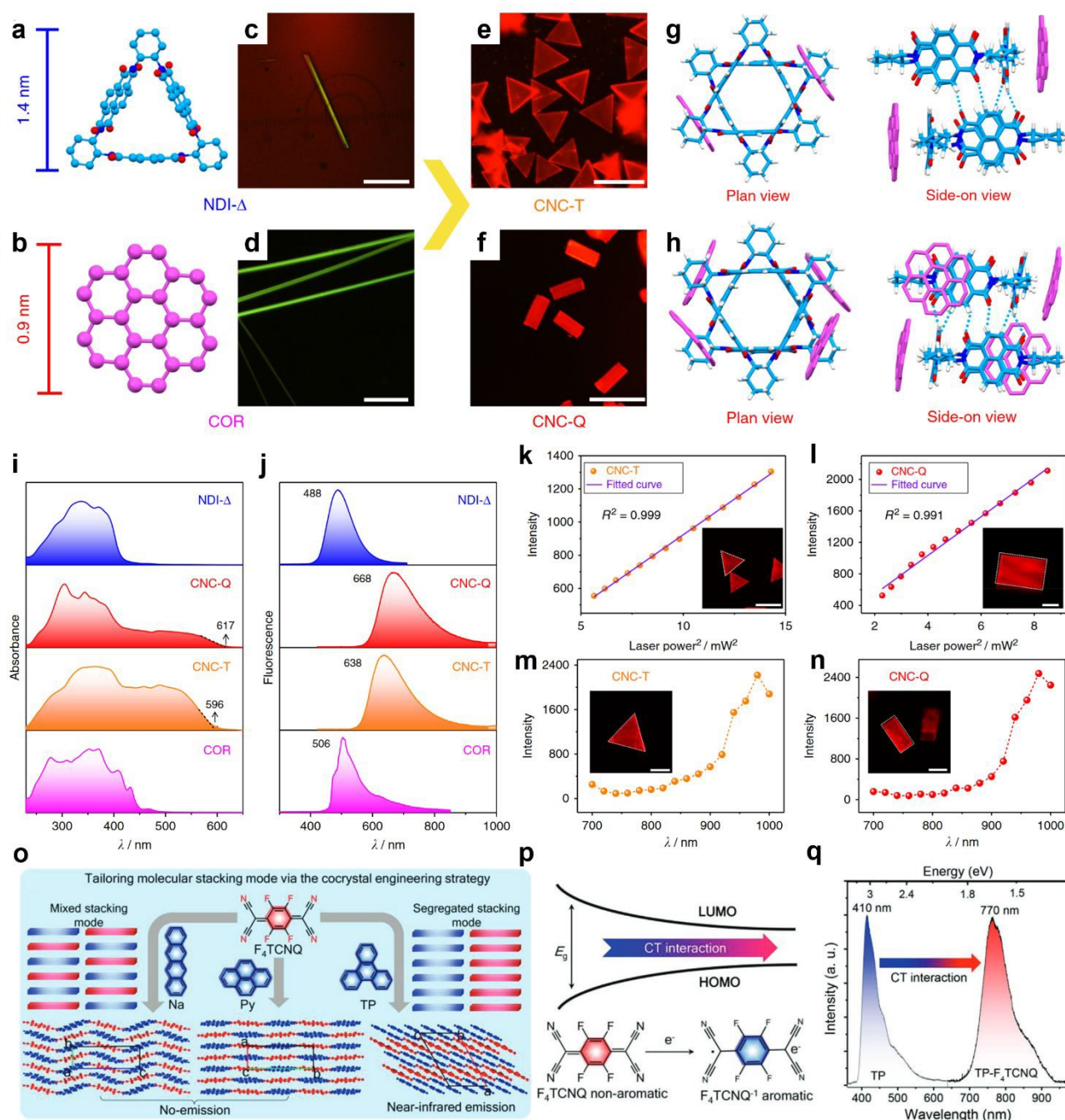
Fig. 5 Donor-acceptor cocrystals for red-shifted and two-photon responsive near-infrared emission. (a, b) Molecular structures and dimensions of NDI-Δ (light blue: C; dark blue: N; red: O) and COR (pink: C). (c, d) Fluorescence microscopy images of needle-like NDI-Δ and COR crystals showing green emission. Scale bars: 20 μm and 40 μm, respectively. (e, f) Fluorescence microscopy images of cocrystals CNC-T (triangular) and CNC-Q (quadrangular), both exhibiting red luminescence. Scale bars: 50 μm. (g, h) Molecular packing diagrams (plan and side views) of CNC-T and CNC-Q, demonstrating distinct face-to-face π-π stacking interactions between NDI-Δ and COR components in the solid state. (i, j) Solid-state absorption and fluorescence spectra of NDI-Δ, CNC-Q, CNC-T, and COR, where cocrystals exhibit pronounced red-shifted emissions due to charge-transfer (CT) interactions. (k, l) Laser power-dependent two-photon excited fluorescence intensity of CNC-T and CNC-Q ( \lambda_{ex} = 1000 nm), fitted with quadratic relationships ( R^2 > 0.99 ). Insets: two-photon fluorescence images; scale bars: 20 μm and 50 μm, respectively. (m, n) Two-photon fluorescence images of CNC-T and CNC-Q. (o) Schematic of the cocrystal engineering strategy, illustrating the transition from mixed stacking mode to segregated stacking mode via the cocrystal engineering strategy, leading to near-infrared emission. (p) Schematic of the charge-transfer interaction, illustrating the transition from F_4TCNQ non-aromatic to F_4TCNQ^{-1} aromatic. (q) Energy level diagram and two-photon fluorescence spectra, illustrating the CT interaction and the resulting red-shifted emission.
