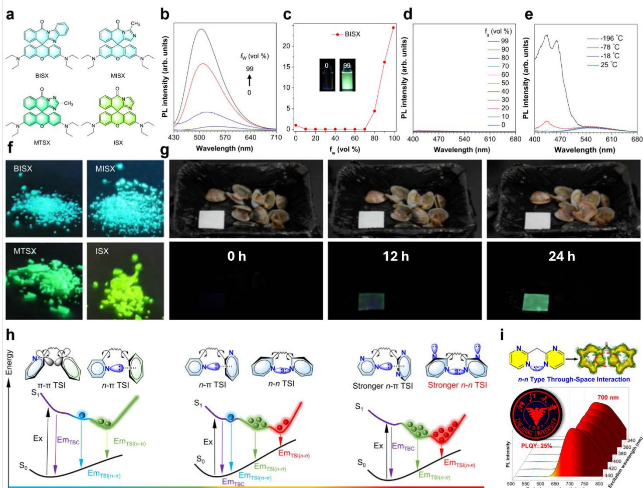
Fig. 1 Aggregation-induced conformationally driven emission changes in nonconjugated systems. (a) Molecular structures of rotor-free Rhodamine B-based AIEgens (BISX, MISX, MTSX, and ISX). The filled colours correspond to their aggregate emission. (b) AIE behavior of BISX: PL spectra in THF/water mixtures with increasing water fractions ( f_w ). c = 1 \times 10^{-5} M; \lambda_{\text{ex}} = 365 nm. (c) Plot of \alpha_{\text{AIE}} ( I/I_0 ) versus f_w . Inset: fluorescence images of BISX in f_w = 0\% and 99\% . (d) PL spectra of BISX in methanol/glycerol mixtures with different glycerol fractions ( f_g ). (e) Temperature-dependent PL spectra of BISX in THF at various temperatures. (f) Fluorescence images of BISX, MISX, MTSX, and ISX aggregates. (g) Biogenic amine detection via fluorescence changes in BISX-loaded sensors after clam exposure for 0, 12, and 24 h. Reproduced from ref. 66 . Copyright © 2024, The Author(s), published by Springer Nature under a CC BY license. (h) Schematic energy diagrams showing different TSIs ( \pi - \pi , n - \pi , and n - n ) and their influence on emission in o-1Py-1Ph, o-2Py, and o-2Md. (i) Structure and AICD isosurface of o-2Md exhibiting sigma-type n - n TSI. Right: excitation-dependent PL spectra and fluorescence image under 365 nm. Reproduced with permission from ref. 67 . Copyright © 2024, Elsevier Inc.
