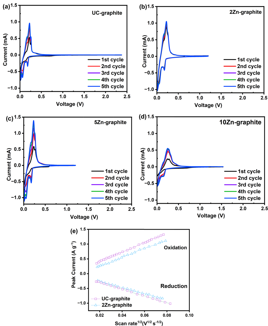
Fig. 3 CV curves of the first five cycles of charge/discharge at 0.1\ mV\ s^{-1} for electrodes made of (a) UC-graphite, (b) 2Zn-graphite, (c) 5Zn-graphite, (d) 10Zn-graphite, and (e) peak current vs. the square root of the scan rate for graphite electrodes.
