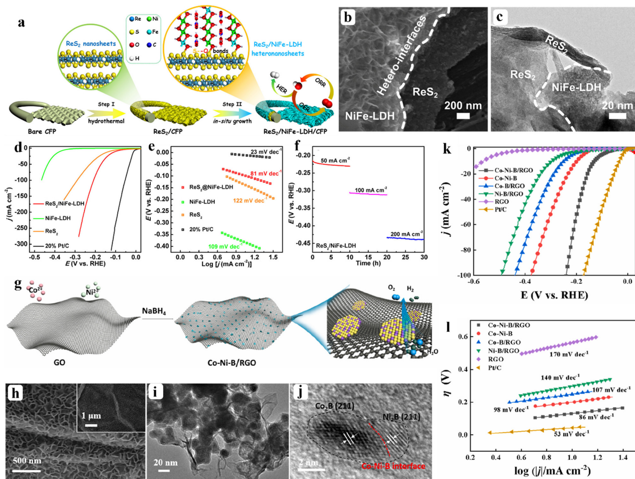
Fig. 4 (a) Schematic illustration of synthesis process, (b) field emission scanning electron microscope (FE-SEM) image, (c) TEM image of the ReS 2 /NiFe-layered double hydroxide (LDH) heteronanosheets, (d) HER polarization curves, and (e) polarization curve-derived Tafel slopes of the ReS 2 /NiFe-LDH heteronanosheets, NiFe-LDH, ReS 2 , and 20% Pt/C in Ar-saturated 1 M KOH solution, (f) Chronopotentiometry curves of the ReS 2 /NiFe-LDH heteronanosheets at various current densities of 50, 100, and 200 mA cm -2 , respectively. Reprinted with permission. 65 Copyright 2021, American Chemical Society. (g) Schematic illustration for the Co-Ni-B/reduced graphene oxide (RGO) fabrication, (h) SEM image, (i) TEM, (j) HRTEM of Co-Ni-B/RGO, (k) HER polarization curves, and (l) corresponding Tafel plots of Co-Ni-B/RGO compared with those of RGO, Co-B/RGO, Ni-B/RGO, Co-Ni-B, and Pt/C. Reprinted with permission. 66 Copyright 2024, Elsevier.
