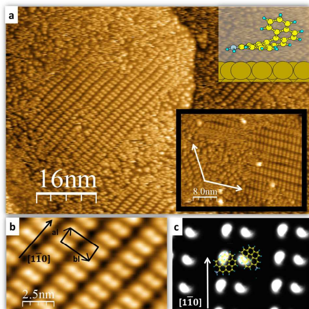
Fig. 2 STM images of M-AH on Au(111). (a) 90%ML coverage, the grow direction of the 120° rotamers is shown by the white arrows in the lower inset. (-2 V,10pA), the upper inset shows the preferential adsorption geometry obtained by DFT (b) 90% ML coverage, a low pass filtered STM image with the unit cell ( a=1.1 , b=2.2 nm)(-2V,10pA), (c) Simulated STM image of the most stable structure (-S7,ESI)
