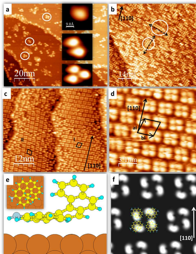
Fig.1 STM images of M-AH on Cu(100). (a) low coverage, insets and circles show the single molecules, dimers, trimers and tetramers diffusing on the surface (-2V, 50 pA). (b) 60% ML coverage, the circles and arrows indicate the formation of double rows (-2V,15pA)(c,d) 90%ML coverage, in black the unit cells for the 90° rotamers (I,II) (a1= b1= 2.4nm) (-2.2V,10pA), (e)DFT model of the single molecules on Cu(100), top and lateral view, (f) Simulated image of calculated cell (S3, ES1)
