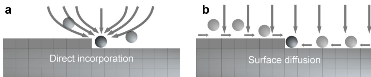
Fig. 6. Schematic of two pathways from solution to kinks: direct incorporation, in a , and via adsorption on the terraces followed by diffusion towards the steps in b . Arrows indicate supply fluxes of solute, depicted as spheres, towards the steps.
