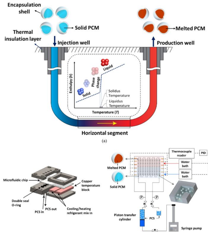
Figure 3. Lab-on-a-chip analysis of processes relevant to geothermal energy. A closed-loop geothermal system (a) is a closed system, and can benefit from specialized working fluids. The work highlighted here employs LoC methods (b) to assess the potential for a microencapsulated phase change slurry as a working fluid, with testing at temperatures, pressures and shear-rates relevant to large scale operations 121 .
