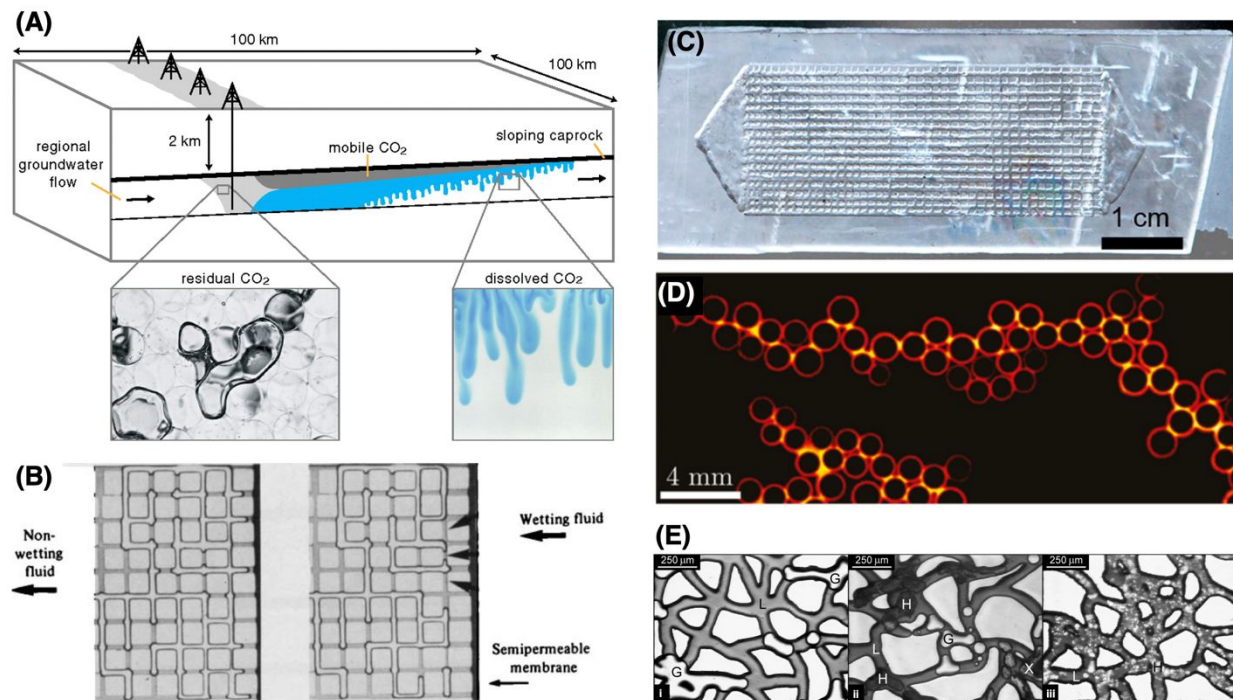
Figure 1. Lab-on-a-chip visualization of multiphase flow processes relevant to carbon sequestration. (A) Schematic of subsurface CO 2 storage describing the two key trapping mechanisms that contribute to storage capacity, residual trapping (left inset) and solubility trapping (right) 10 . (B) Snap-off of wetting films leading to capillary trapping of gas during imbibition 11 . (C) Geometrically and chemically representative real-rock micromodel for reservoir engineering studies 12 . (D) Snapshot from strong imbibition illustrating invasion by corner flow: the invading fluid advances by coating the perimeters of the posts rather than by filling the pore bodies; pendular rings link the coated posts, forming chains 13 . (E) Snapshots of methane hydrate
