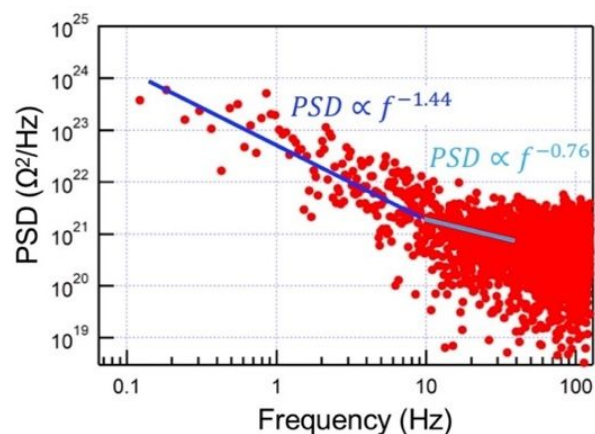
Fig. 5 Power spectral density (PSD) measured by applying a constant bias of 4 V to a \text{Ag}_2\text{S} island network.
