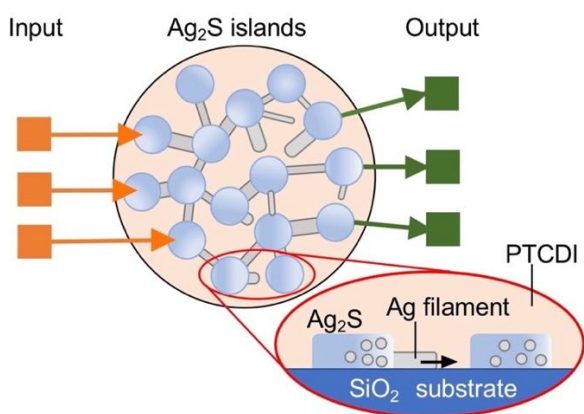
Fig. 1 Schematic of a \text{Ag}_2\text{S} island network-based reservoir. Ag filaments grown from \text{Ag}_2\text{S} islands make conductive channels in the network.
