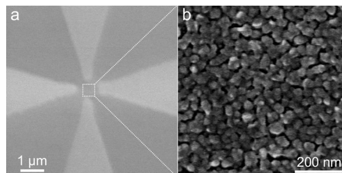
Fig. 2 (a) SEM image of four electrodes surrounding the \text{Ag}_2\text{S} island network. (b) Magnified SEM image of \text{Ag}_2\text{S} islands.
