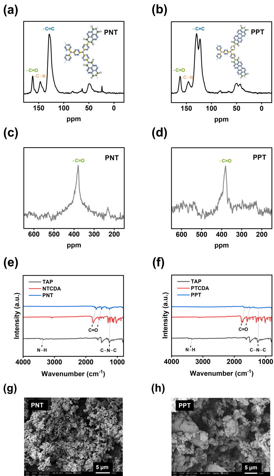
Fig. 1 Material characterizations for the PNT and PPT: (a-b) ^{13}\text{C} solid-state NMR, (c-d) ^{17}\text{O} solid-state NMR, (e-f) FTIR spectra, (g-h) SEM images.
