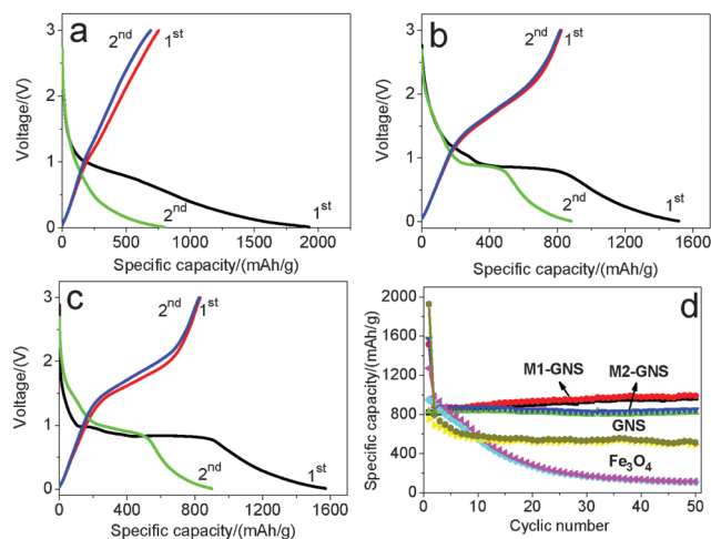
Fig. 9 The initial two charge/discharge curves of (a) original GNS, (b) M1-GNS and (c) M2-GNS, and (d) cycling performance of M1-GNS, M2-GNS, GNS, and \text{Fe}_3\text{O}_4 nanoparticles at the current density of 50\text{ mA g}^{-1} .
