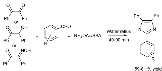
Scheme 27 Synthesis of 2,4,5-triaryl-1H-imidazoles from benzil or benzoin or benzylmonoxime, aldehyde and ammonium acetate in the presence of silica sulphuric acid (SSA) catalyst.
