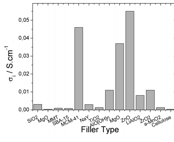
Fig. 4 Ionic conductivity for different filler types.
