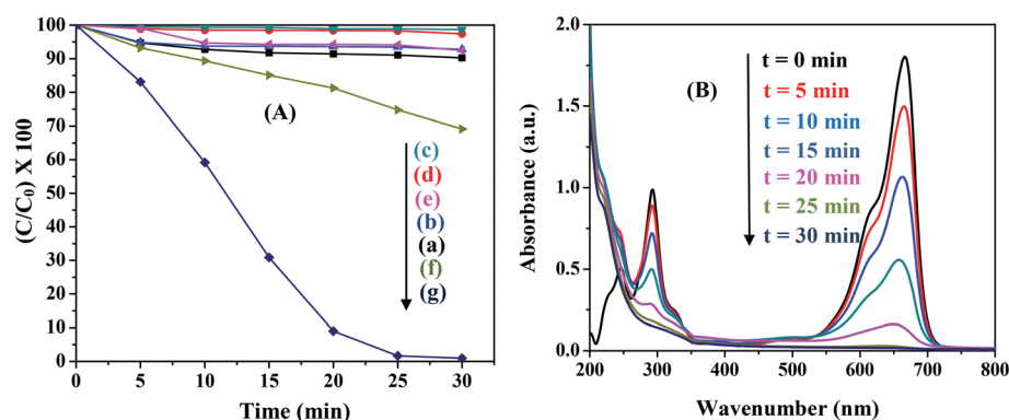
Fig. 6 (A) Control experiments for photocatalytic degradation in the presence of \text{NiFe}_2\text{O}_4 . The reaction conditions are: (a) MB + light, (b) MB + \text{H}_2\text{O}_2 + dark, (c) MB + \text{H}_2\text{O}_2 + light, (d) MB + ferrite + dark, (e) MB + ferrite + light, (f) MB + ferrite + \text{H}_2\text{O}_2 + dark, and (g) MB + ferrite + \text{H}_2\text{O}_2 + light. (B) Change in absorption spectra of MB with time in the presence of \text{NiFe}_2\text{O}_4 ( 0.5 \text{ g L}^{-1} , pH-2.5, \text{H}_2\text{O}_2 -8 mM).
