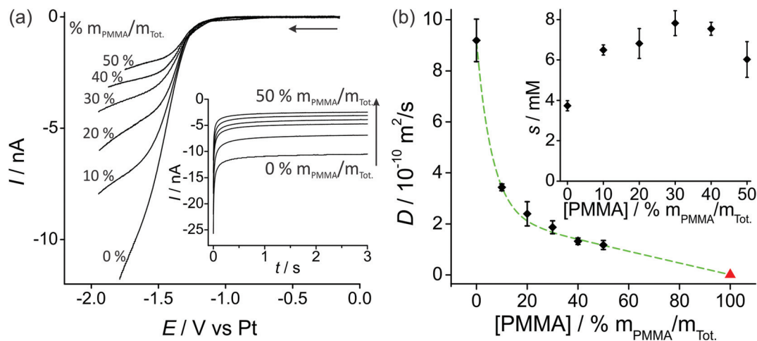
Fig. 2 (a) Linear sweep voltammetry (10 mV s -1 ) for 100 vol% O 2 in PMMA-[C 2 mim][NTf 2 ] mixtures at 0–50% m PMMA /m Tot , on a platinum microdisk electrode (radius 7.44 μm). The inset shows the corresponding chronoamperometric transients. (b) Plot of diffusion coefficient ( D ) of O 2 vs. [PMMA] (the red triangle for pure PMMA, i.e. 100% m PMMA /m Tot is taken from the literature 22 ). The inset shows oxygen solubilities s vs. [PMMA]. D and s were obtained by fitting chronoamperometric transients to the Shoup and Szabo equation. 21
