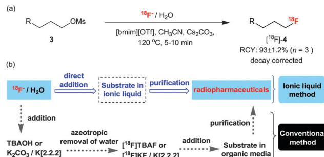
Scheme 15 (a) ^{18}\text{F} -radiofluorination in IL [\text{bmim}][\text{OTf}] . (b) A schematic comparison of the conventional ^{18}\text{F} labeling process and the IL-based process.
