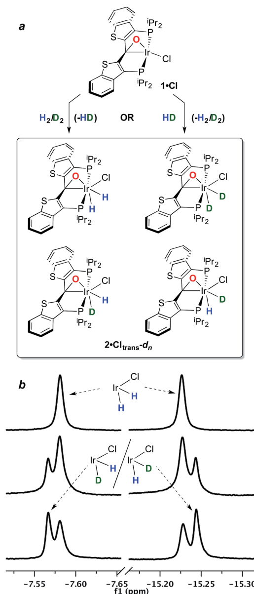
Fig. 1 (a) Reaction of compound 1-Cl with either a 1 : 1 mixture of H_2/D_2 or pure HD leads to the mixture of isotopologues of compound 2\cdot Cl_{trans} . (b) Hydride region of the ^1H\{^{31}P\} NMR spectrum of pure 2\cdot Cl_{trans} (top), the reaction mixture when 1-Cl is treated with H_2/D_2 (middle) and the reaction mixture when 1-Cl is treated with HD (bottom). Note that, while the outer resonances in each pair are due to the 2\cdot Cl_{trans-d_1} isotopomers, we have not made absolute assignments for these resonances.
