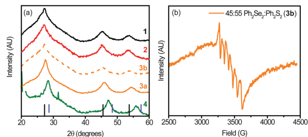
Fig. 4 (a) XRD patterns of samples 1 , 2 , 3a , 3b , and 4 . The patterns indicate zinc-blend structure and the broadness of the peaks indicates small NC diameters or domains. As the amount of S increases, the peaks shift to larger angles. The black lines at the bottom of the figure represent the positions of bulk ZnSe and the blue lines represent those of bulk ZnS. (b) EPR spectrum of 3b showing a splitting pattern with 6 peaks and a hyperfine coupling constant of 66.2 G.
