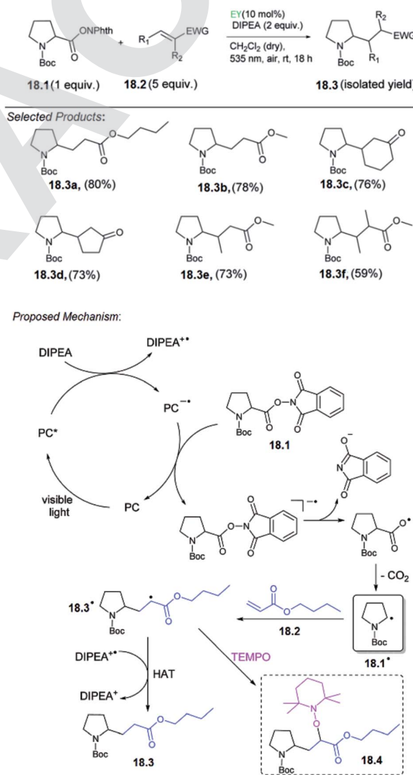
Scheme 18 Decarboxylative alkylation.
