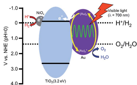
Scheme 1 Expected reaction mechanism for the production of \text{H}_2 and \text{O}_2 from water over a \text{Au/TiO}_2\text{-NiO}_x sample.
