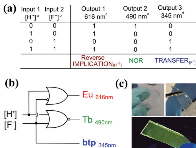
Fig. 24 (a) The truth table of the logic functions. a [H^+] = 2 mM; b [F^-] = 1 mM. (b) A circuit diagram of the observed logic gate functions. c Phosphorescence. d Fluorescence. (c) Images of Eu 1.3 and Tb 2.3 based gels when swelled in H_2O (left) and CH_3OH (right) under ambient light, after drying and irradiation at 254 nm, demonstrating the (0,0) state. Reproduced with small alterations from ref. 45 with permission from Royal Society of Chemistry, copyright 2015.
