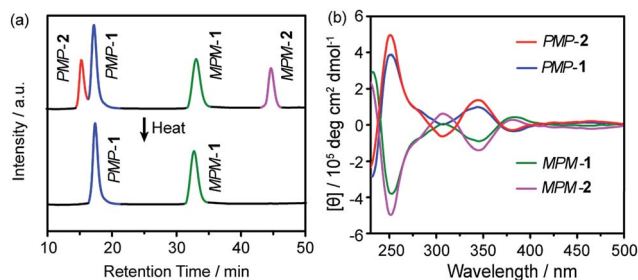
Fig. 2 Chiral-HPLC and CD analyses of 1 and 2 . (a) Chiral HPLC spectra of the kinetic products (top) synthesised at ambient temperature revealing two pairs of diastereoisomers, ( i.e. , MPM -1 and PMP -1, PMP -2 and MPM -2) that changed into the thermodynamic products ( MPM -1 and PMP -1) when heated at 50 °C for five days (bottom). (b) CD spectra of PMP -2, MPM -1, MPM -1 and MPM -2 (10 μM) in dichloromethane.
