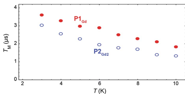
Fig. 7 Temperature dependence of the quantum coherence time T_{\text{M}} for \text{P1}_{\text{Gd}} (red full dots) and \text{P2}_{\text{Gd2}} (blue empty dots), as measured at 344 mT at 9.37 GHz in a 1 : 1 mixture of dichloromethane and toluene.
