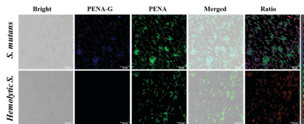
Fig. 5 Fluorescence images of Streptococcus mutans (ratio = 0.46) and Hemolytic streptococcus (ratio = 0.04) in the presence of potential inhibitor EGCG (50 µM). PENA-G \lambda_{\text{ex}} 405/ \lambda_{\text{em}} 415–465 nm, PENA \lambda_{\text{ex}} 405/ \lambda_{\text{em}} 535–585 nm, Scale bar 10 µm.
