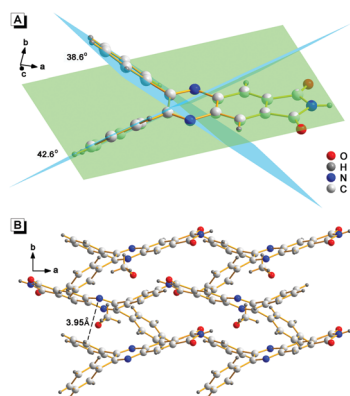
Fig. 2 Crystal structure of 2 . (A) The dihedral angles between the conjugate rigid planes. (B) The packing of 2 in the crystal and the minimum distance between the adjacent conjugate planes.
