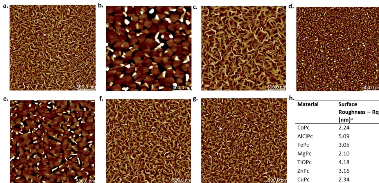
Fig. 5 AFM images ( 2.5\ \mu\text{m} \times 2.5\ \mu\text{m} ) of (a) CoPc (b) AlClPc (c) FePc (d) MgPc (e) TiOPc (f) ZnPc (g) CuPc deposited on heated silicon substrates ( T = 140\ ^\circ\text{C} ) under vacuum (h) surface roughness values (nm) for each film.
