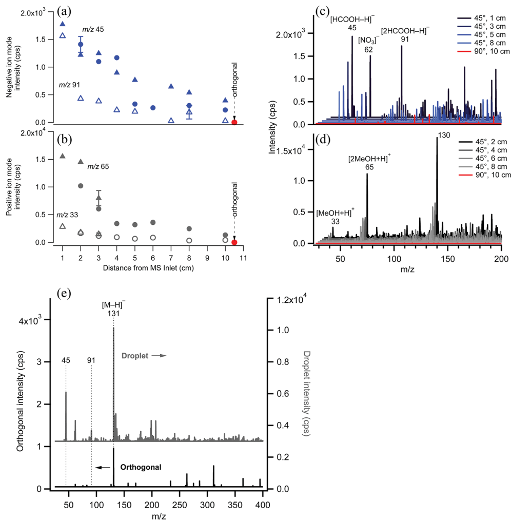
Fig. 4 MS intensity as a function of increasing distance of the nebulizer from the MS inlet for (a) negative ion mode [HCOOH-H]^- solvent peak and (b) positive ion mode solvent peaks [MeOH+H]^+ and [2MeOH+H]^+ and their corresponding ESI mass spectra (c, d). Different symbols represent repeated measurements with slightly different nebulizer position and error bars are 1s standard deviations from replicate measurements. The peak at m/z 130 in (d) is due to an unknown solvent contaminant. (e) Typical ESI-MS mass spectra of solid, bare glutaric acid particles in droplet (grey) and orthogonal (black) modes showing the presence and absence, respectively, of typical solvent peaks.
