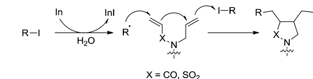
Scheme 26 Indium-mediated radical addition-cyclization-trapping cascade reaction in aqueous media.
