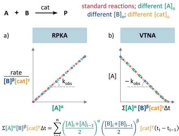
Fig. 6 Straight lines appear in (a) RPKA and (b) VTNA plots when all the changing driving forces are raised to their order of reaction.
