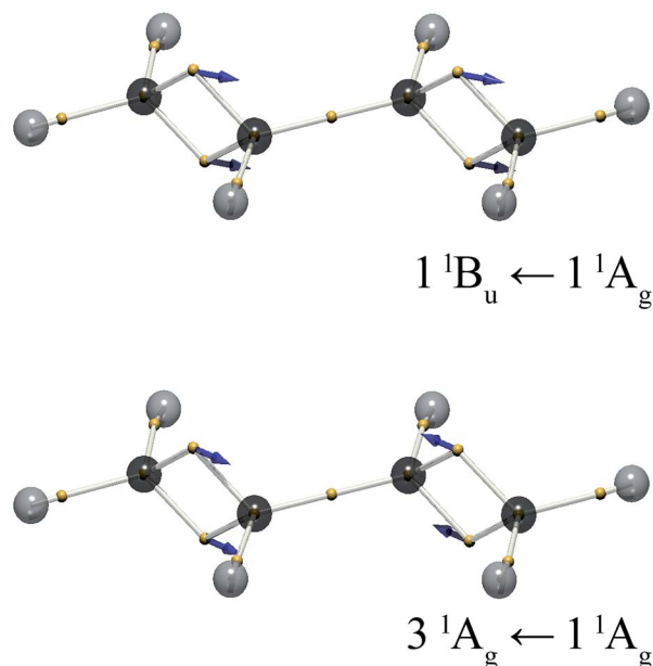
Fig. 5 The electron positions for the mid-point of the vibration, \bar{x} = (\bar{x}_i + \bar{x}_j)/2 , and the displacement vectors \mathbf{x}_{fi} for the 1^1B_u \leftarrow 1^1A_g and 3^1A_g \leftarrow 1^1A_g transitions of trans -butadiene. The vector length is doubled for clarity.
