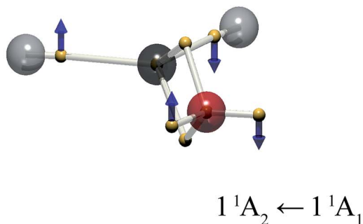
Fig. 4 The electron positions for the mid-point of the vibration, \bar{x} = (\bar{x}_i + \bar{x}_j)/2 , and the displacement vectors \mathbf{x}_{fi} for the wavefunction mixed between the 1^1A_1 (ground), and 1^1A_2 , 2^1A_1 and 1^1B_1 excited states of formaldehyde. The vector length is doubled for clarity.
