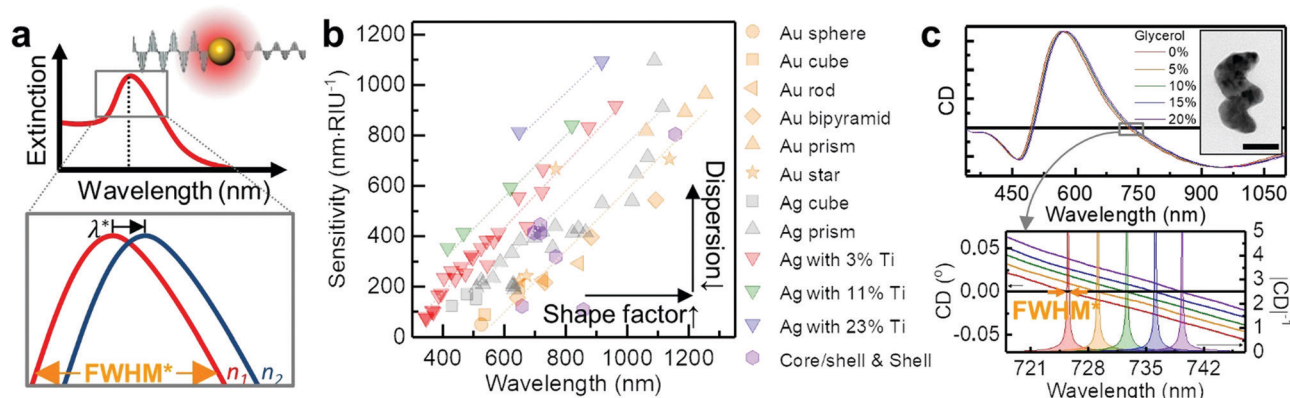
Fig. 3 Plasmonic extinction spectroscopy. (a) Schematic view of plasmonic sensing. Top panel shows the plasmonic resonance of metallic nanoparticles as a function of wavelength. Inset shows a metallic nanosphere interacts with light and generates a detectable absorption peak due to LSPR. The bottom panel shows a zoomed-in region near the peak, illustrating how it shifts in wavelength as the refractive index of the surrounding medium changes n_1 < n_2 . (b) Sensitivities of plasmonic NPs reported in the literature as a function of the peak wavelength in water. The symbols and colours are different for the shapes and the material composition respectively (Au sphere, 80 Au cube, 80 Au rod, 80 Au bipyramid, 80 Au prism, 177 Au star, 80,178,179 Ag sphere, 180,181 Ag cube, 182,183 Ag prism, 180,184,185 core/shell (or shell), 186–190 and Ag–Ti nanohelices 85 ). (c) Circular dichroism (CD) spectra of Ag–Ti nanohelices in media of five different refractive indices (red: 0%, orange: 5%, green: 10%, blue: 15% and violet: 20% glycerol–water mixtures) over the full spectral range. Inset shows the TEM image of a single Ag–Ti nanohelix (scale bar 50 nm). The bottom panel shows a detailed plot of the resonance shifts at zero-crossing. The filled curves represent |CD|^{-1} . Adapted from ref. 85 with permission. Copyright 2016 Springer Nature.
