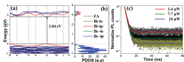
Fig. 3 (a) The electronic band structures and (b) projected density of states (PDOS) of \text{FA}_3\text{Bi}_2\text{Br}_9 calculated at the GGA/PBE level of theory. (c) The time-resolved PL of \text{FA}_3\text{Bi}_2\text{Br}_9 QDs under different excitation intensities.
