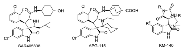
Fig. 1 Spiro-oxindoles SAR405838 and APG-115, 16,17 which are currently under clinical trials, and dispiro-oxindole KM-140 have successfully completed preclinical studies. 10,19
