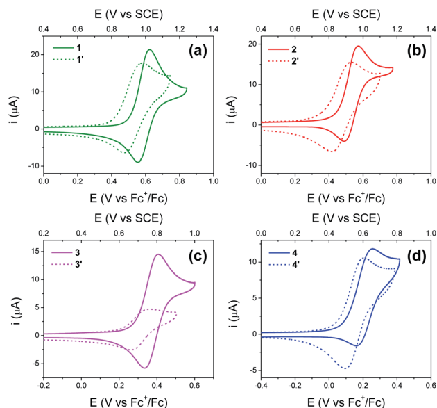
Fig. 4 (a–d) Cyclic voltammograms of BIPs 1'–4' (dashed lines). The cyclic voltammograms of analogous BIPs 1–4 (solid lines) are included for comparison. Concentration: 1 mM of the indicated compound, 0.5 M TBAPF 6 supporting electrolyte in dry acetonitrile. WE: glassy carbon. Pseudo RE: Ag wire (ferrocene as internal reference). CE: Pt wire. Scan rate, 100 mV s −1 . Compound 3' has low solubility in acetonitrile.
