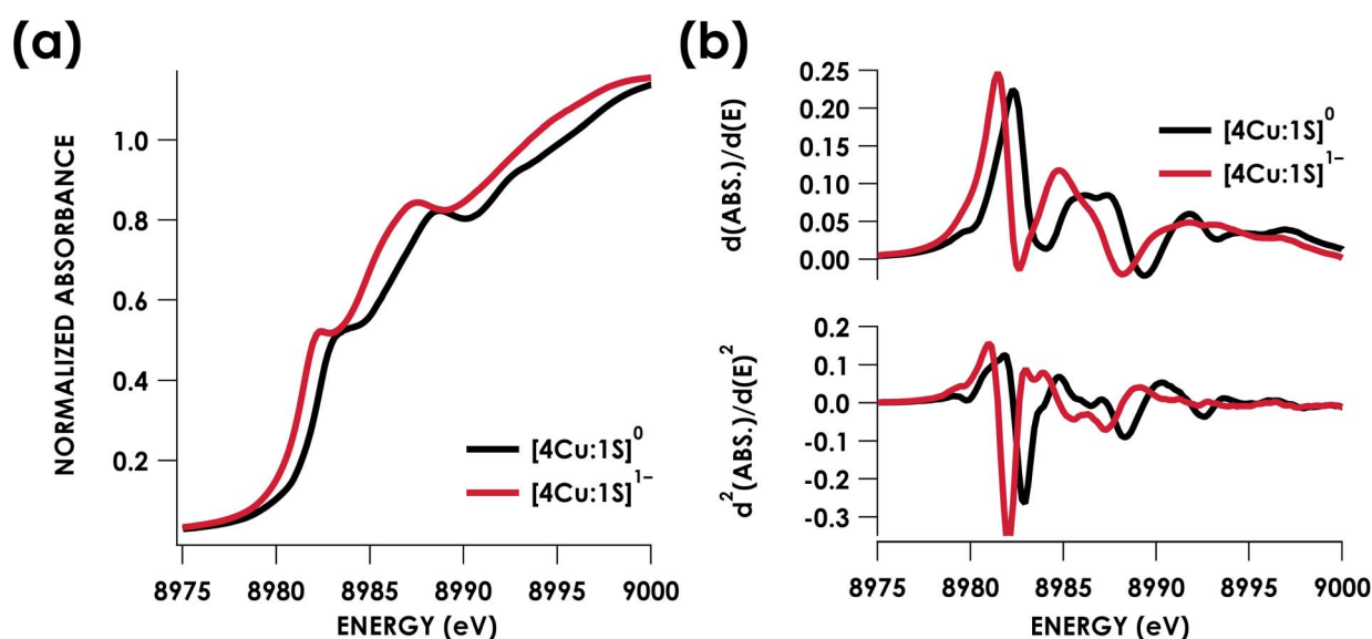
Fig. 3 (a) Cu K-edge XAS spectra obtained for the [4Cu:1S] 0/1- redox couple. (b) First (top) and second (bottom) derivative Cu K-edge XAS spectra. Isoenergetic pre-edge ( 1s \rightarrow 3d ) excitations are evident in the second-derivative spectra at 8979.8 eV. Rising edge inflection points occur at 8982.3 and 8985.9 eV for [4Cu:1S] 0 and 8981.5 and 8984.8 eV for [4Cu:1S] 1- .
