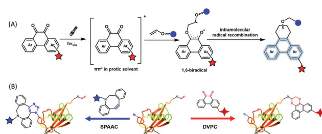
Fig. 2 (A) Visible-light driven bioorthogonal dione–vinyl ether photocycloaddition (DVPC) reaction via the PeT pathway; (B) orthogonal protein labelling achieved by SPAAC and DVPC that are orthogonal to each other.
