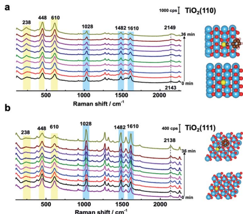
Fig. 4 (a) SHINER Spectra of N719 adsorbed on a rutile \text{TiO}_2(110) surface with 405 nm laser illumination. The right shows the DFT simulated optimized structures of the \text{Ph-N}=\text{C}=\text{S} group (top) and S atom (below) adsorbed on rutile \text{TiO}_2(110) . (b) SHINER Spectra of N719 molecules adsorbed on a rutile \text{TiO}_2(111) surface with 405 nm laser illumination. Spectra were collected every 4 minutes. The right shows the DFT simulated optimized structures of the \text{Ph-N}=\text{C}=\text{S} group (top) and S atom (below) on rutile \text{TiO}_2(111) .
