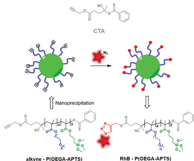
Fig. 32 P(POEGA-APT) BCP obtained by RAFT polymerization using a clickable CTA, allowing labeling by RhB-azide.
