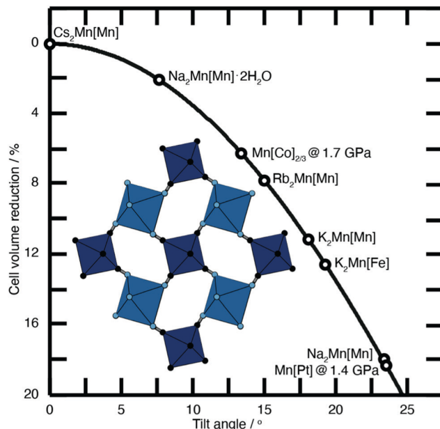
Fig. 2 Approximate link between magnitude of correlated tilts and volume reduction in the PBA structure type. The solid line illustrates the geometric result for volume reduction -\Delta V/V \approx 6r[1 - \cos(\phi)] , where the 'tilt angle' \phi is the average distortion of \text{P}\cdots\text{R}-\text{C} and \text{R}\cdots\text{P}-\text{N} angles, and r is the average ratio of the \text{P}-\text{N}/\text{R}-\text{C} bond lengths to the \text{P}\cdots\text{R} distance. 11,18,21,22 Included in the bottom left is an illustration of one representative tilt distortion. We include the positions of a variety of PBAs discussed in the text. Note, for example, that decreasing A-site cation radius favours larger tilts, as seen for the family \text{A}_2\text{Mn}[\text{Mn}] ( \text{A} = \text{Cs}, \text{Rb}, \text{K}, \text{Na} ).
