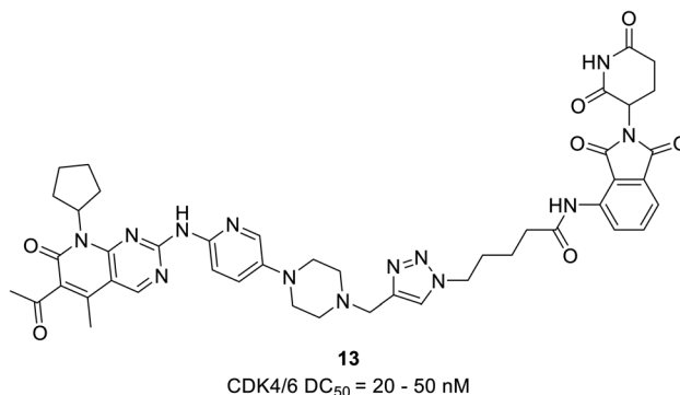
Fig. 19 Palbociclib-based PROTAC 13 as dual CDK4/6 degrader.
