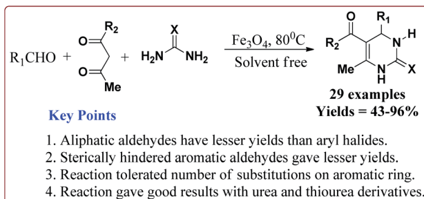
Scheme 33 Fe 3 O 4 nanocatalyst catalyzed Biginelli reactions.
