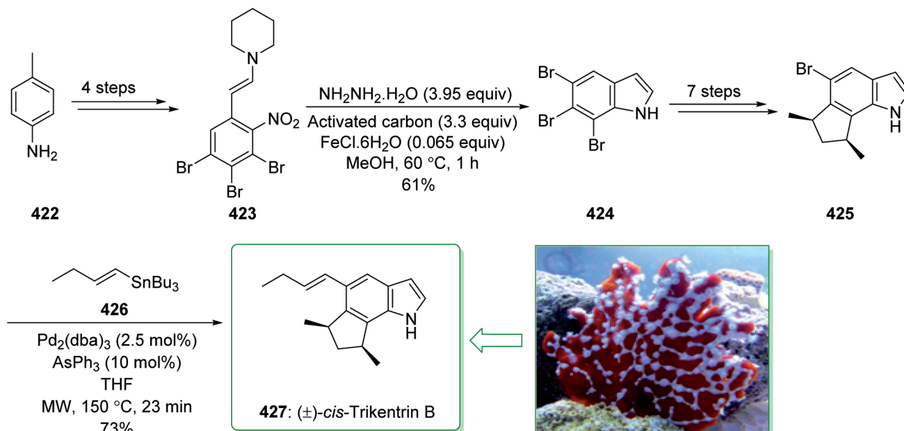
Scheme 59 Total synthesis of ( \pm )- cis -trikentrin B (427).
